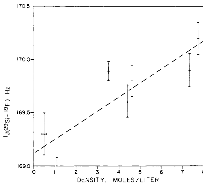
Figure 2. Experimental values of {}^1J({}^{29}\text{Si}-{}^{19}\text{F}) coupling constant in SiF 4 in the gas phase plotted as a function of the density in moles per liter. The dashed line corresponds to the linear least-squares fit of the experimental data.
